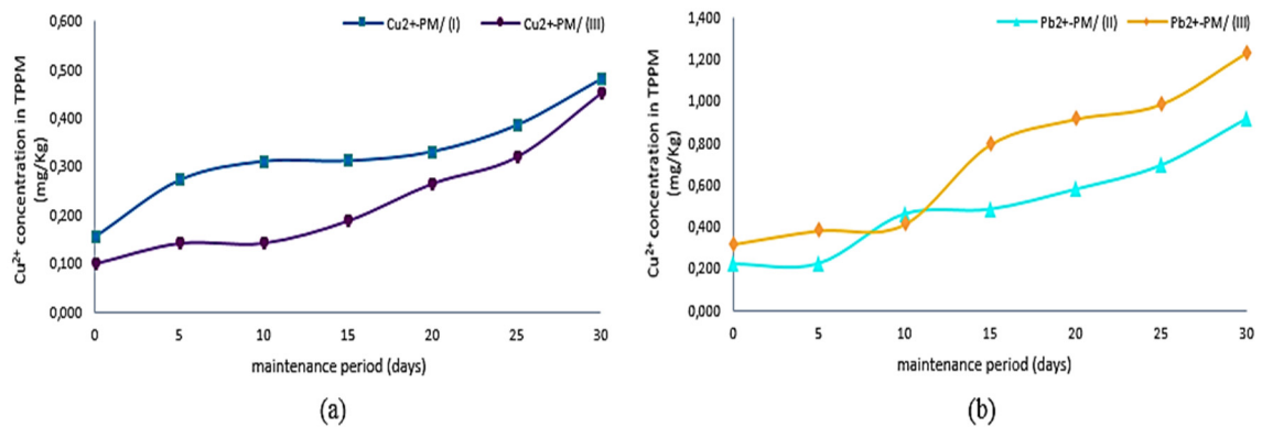
Fig. 5: Comparison of the adsorption concentrations of \text{Cu}^{2+} and \text{Pb}^{2+} pollutants in TPPM. (a) \text{Cu}^{2+} in Treatment I vs. Treatment III and (b) \text{Pb}^{2+} in Treatment II vs. III.
